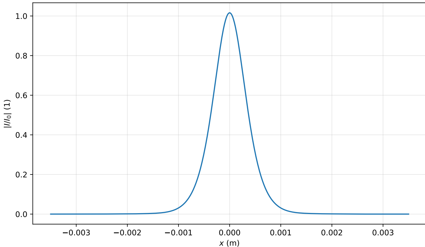
Intensity profile I(x, y = 0, z = 3.344m)/I_0 , P_{in}=0.8P_{cr} , artificial time
